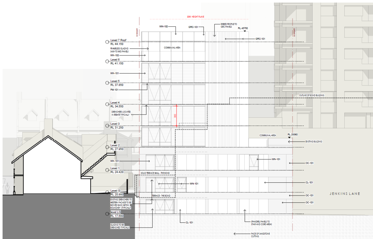
West Elevation
